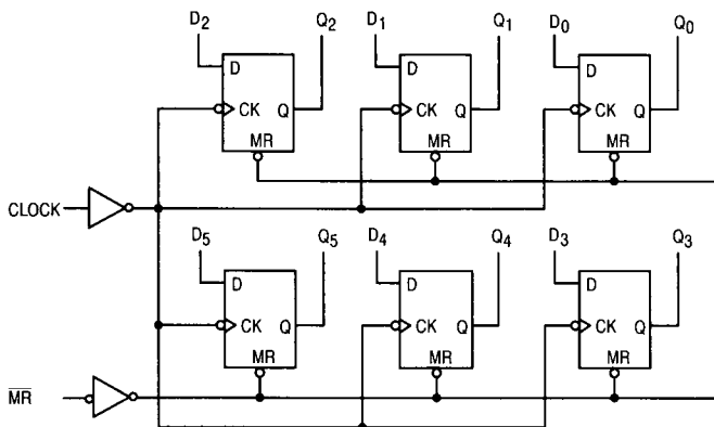
LOGIC DIAGRAM
