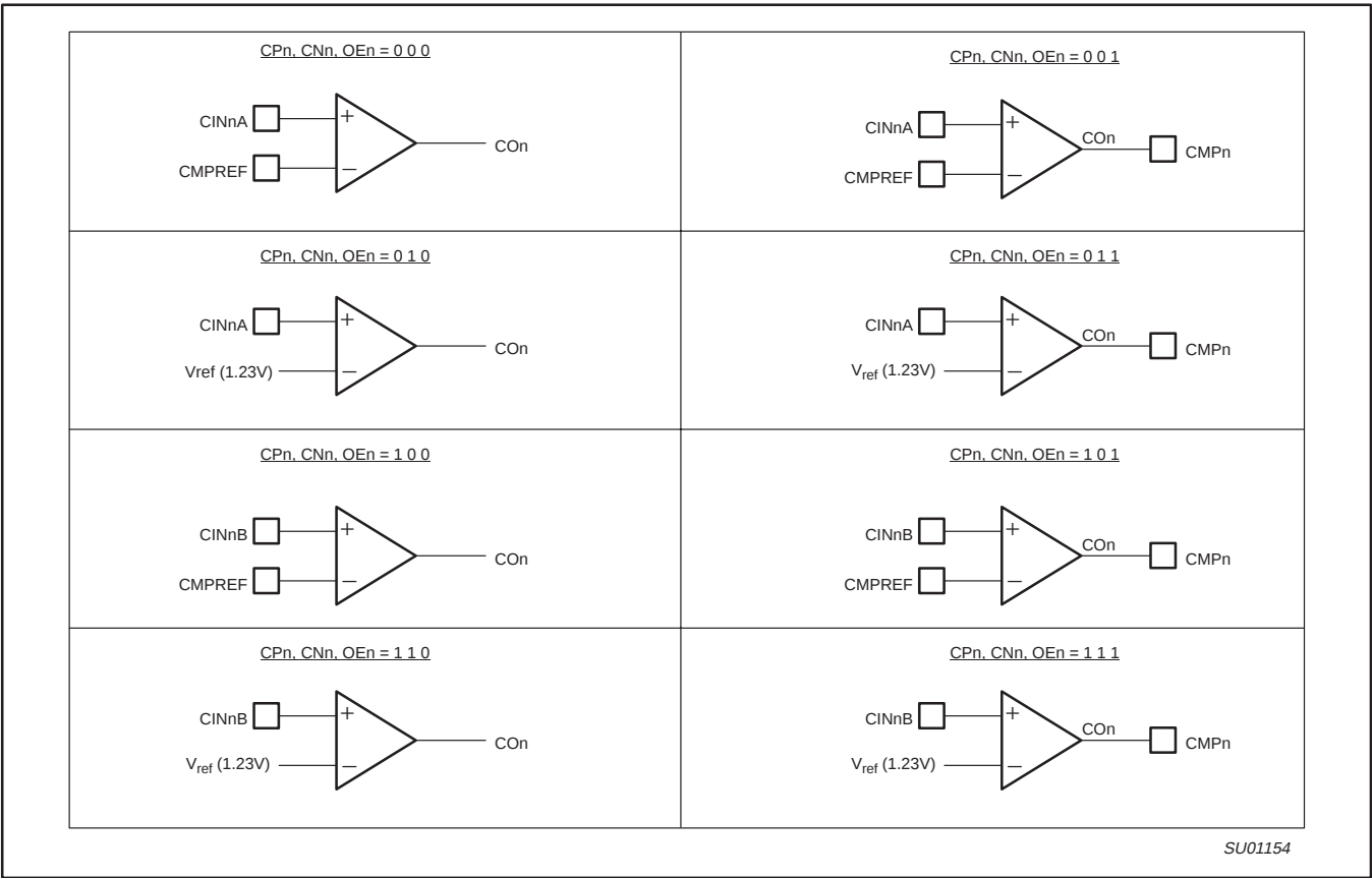
Figure 6. Comparator Configurations
