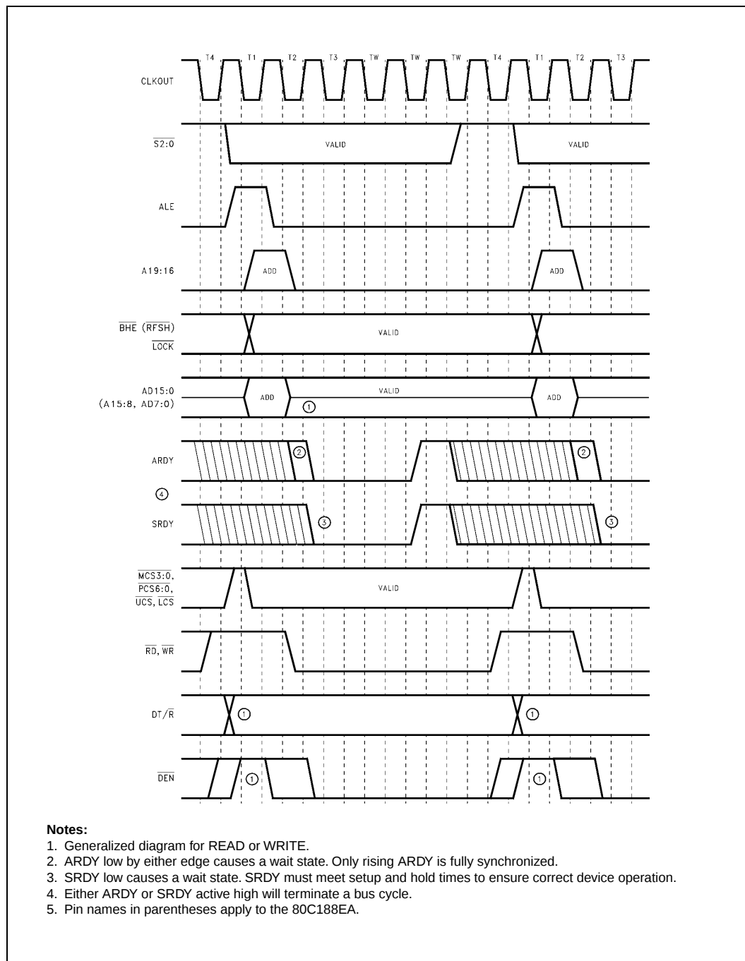
Figure 19. Ready Waveform
