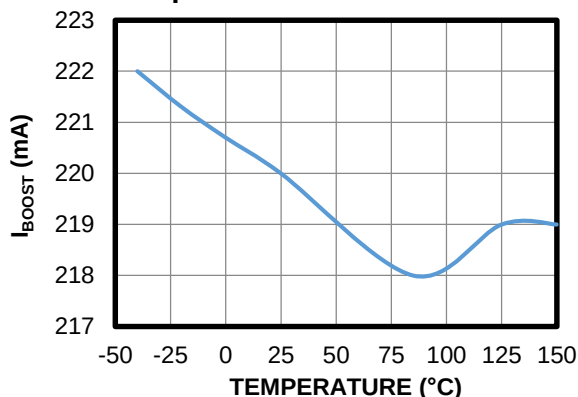
Boost Current Limit vs. Temperature
