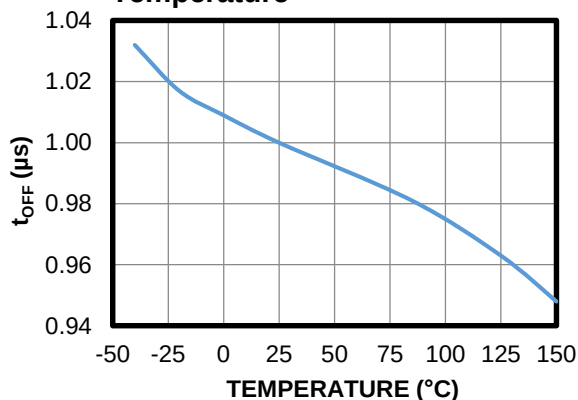
Gate Turn-Off Delay Time vs. Temperature
