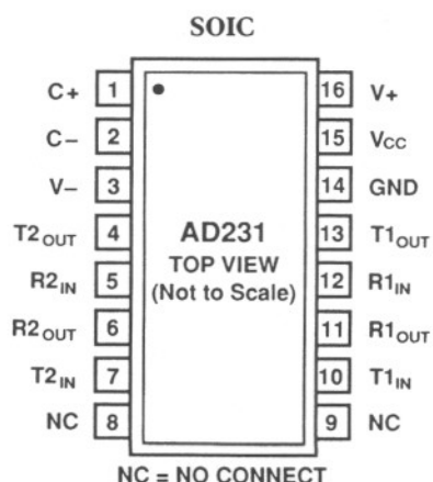
Figure 3. AD231 DIP & SOIC Pin Configurations
