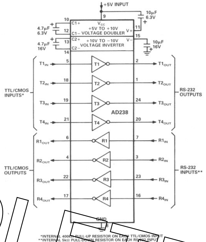
Figure 18. AD238 Typical Operating Circuit
