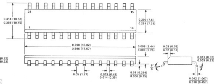
28-Lead SOIC (R-28)
