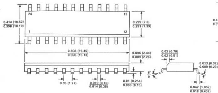
24-Lead SOIC (R-24)
