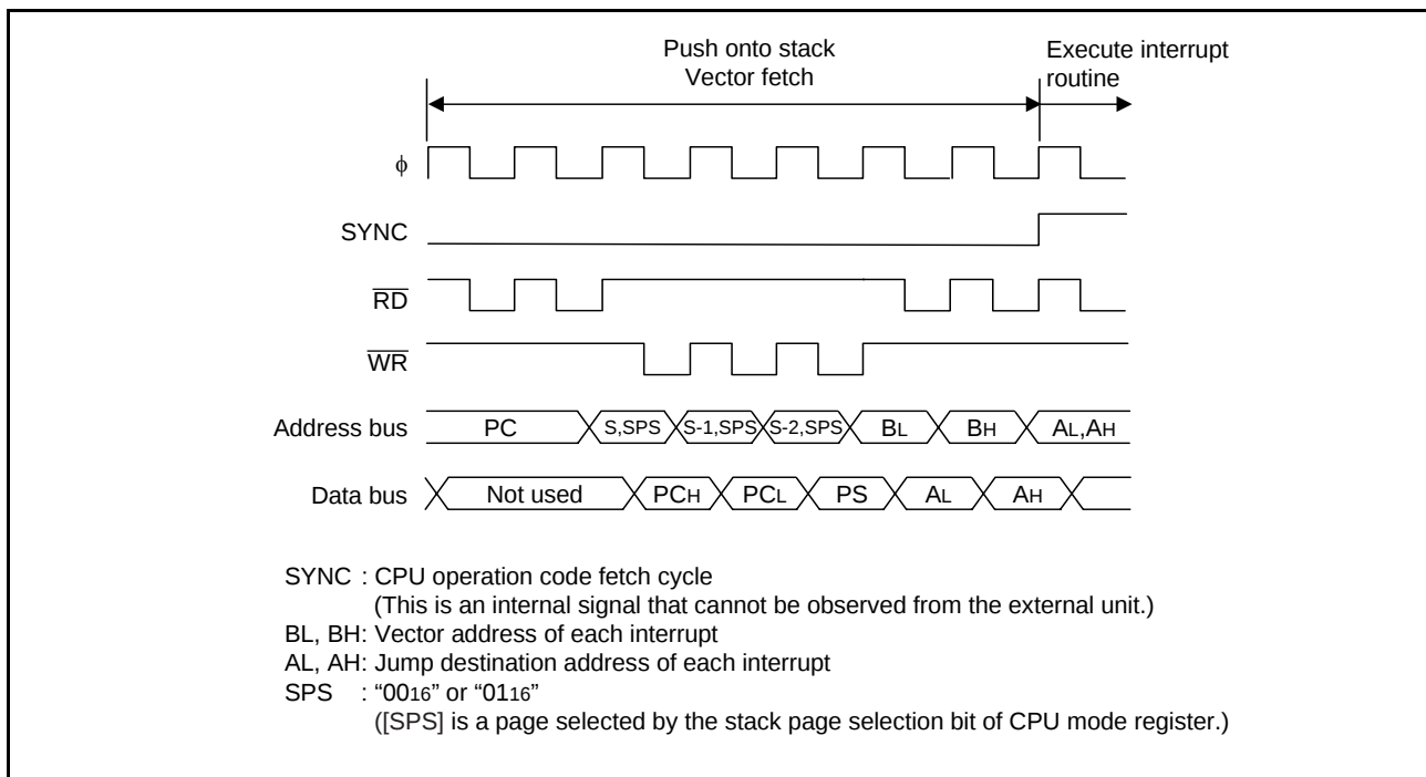
Fig 21. Interrupt sequence
