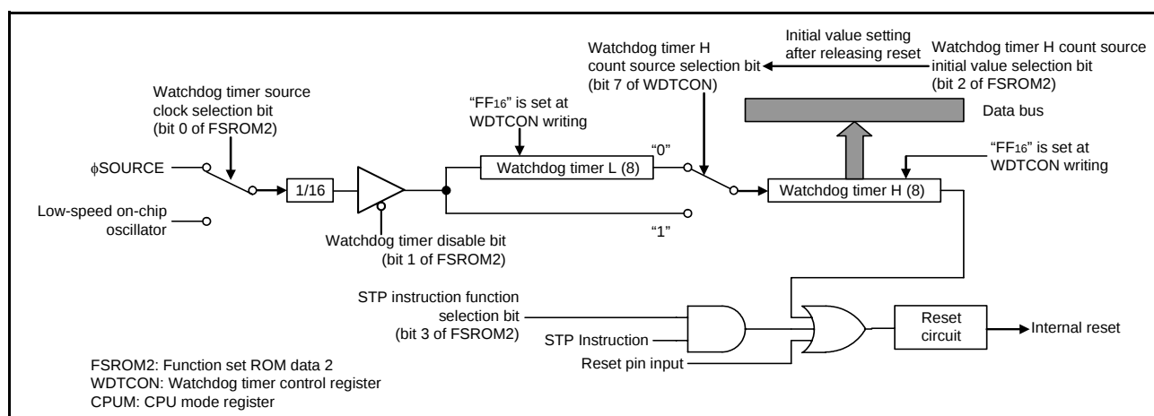
Fig 55. Block diagram of watchdog timer
