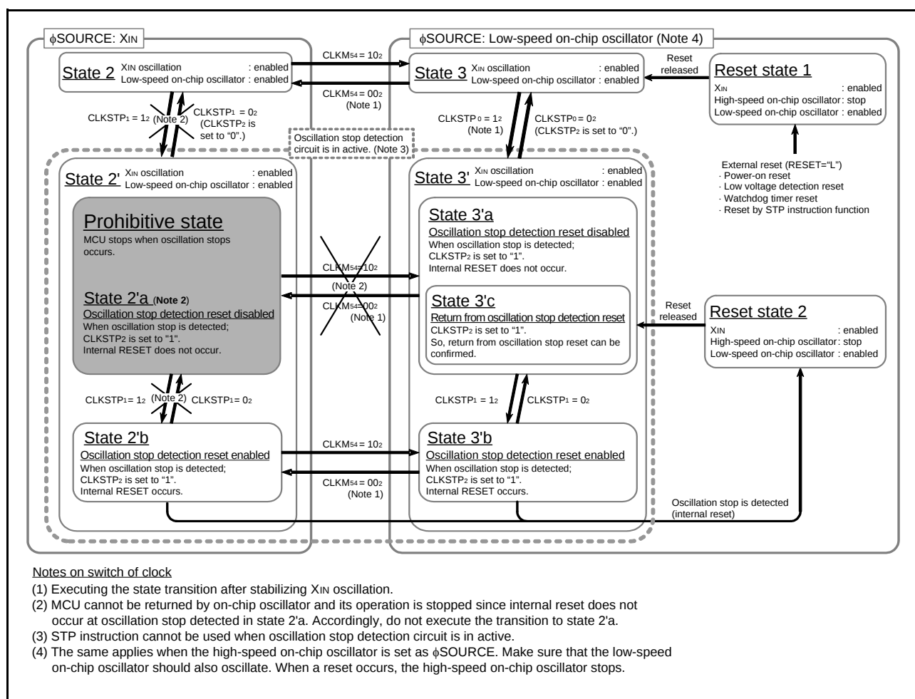
Fig 68. State transition of oscillation stop detection circuit
