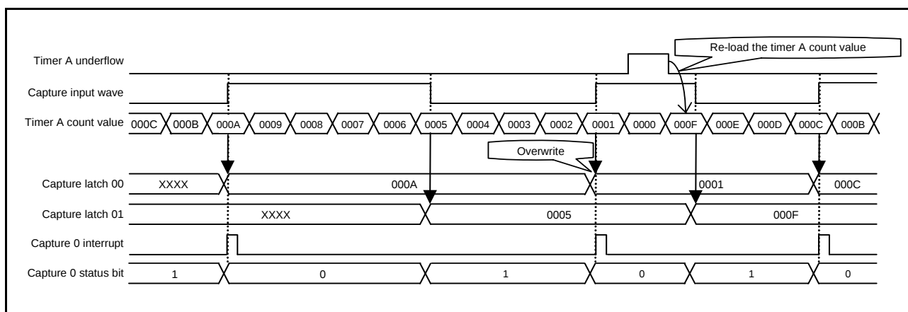
Fig 43. Capture input waveform (capture interrupt edge selection bit = "rising edge")
