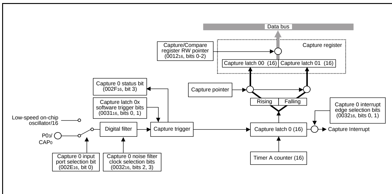
Fig 42. Block diagram of capture channel 0
