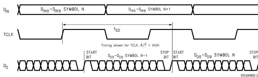
FIGURE 3. Serializer Delay
