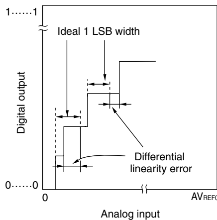
Figure 14-16. Differential Linearity Error
