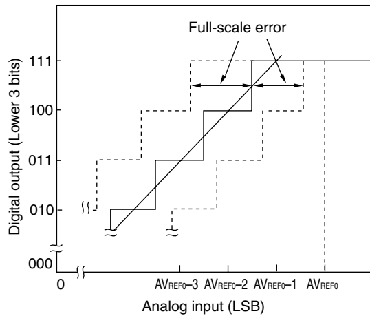
Figure 14-15. Full-Scale Error
