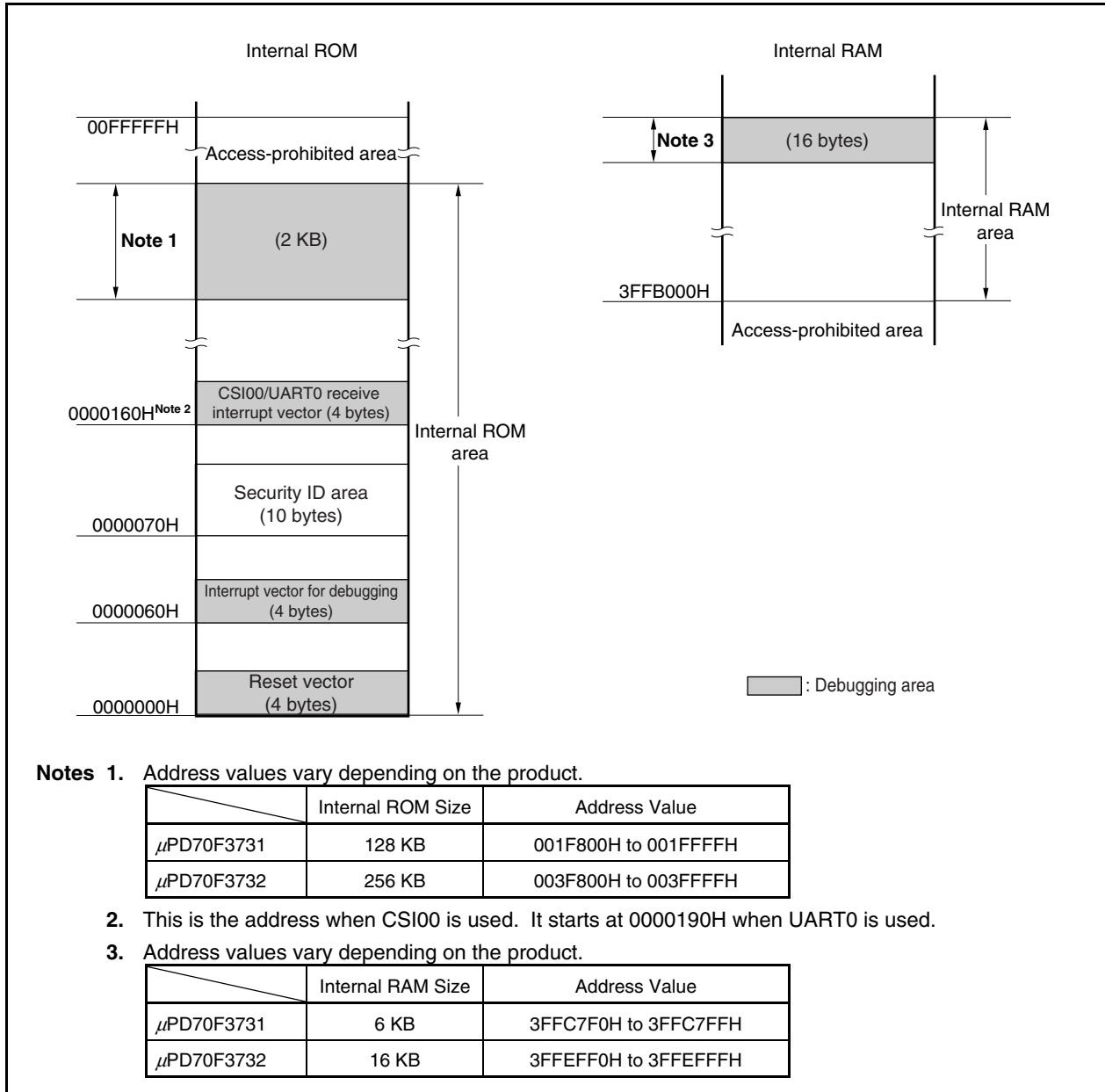
Figure 27-2. Memory Spaces Where Debug Monitor Programs Are Allocated
