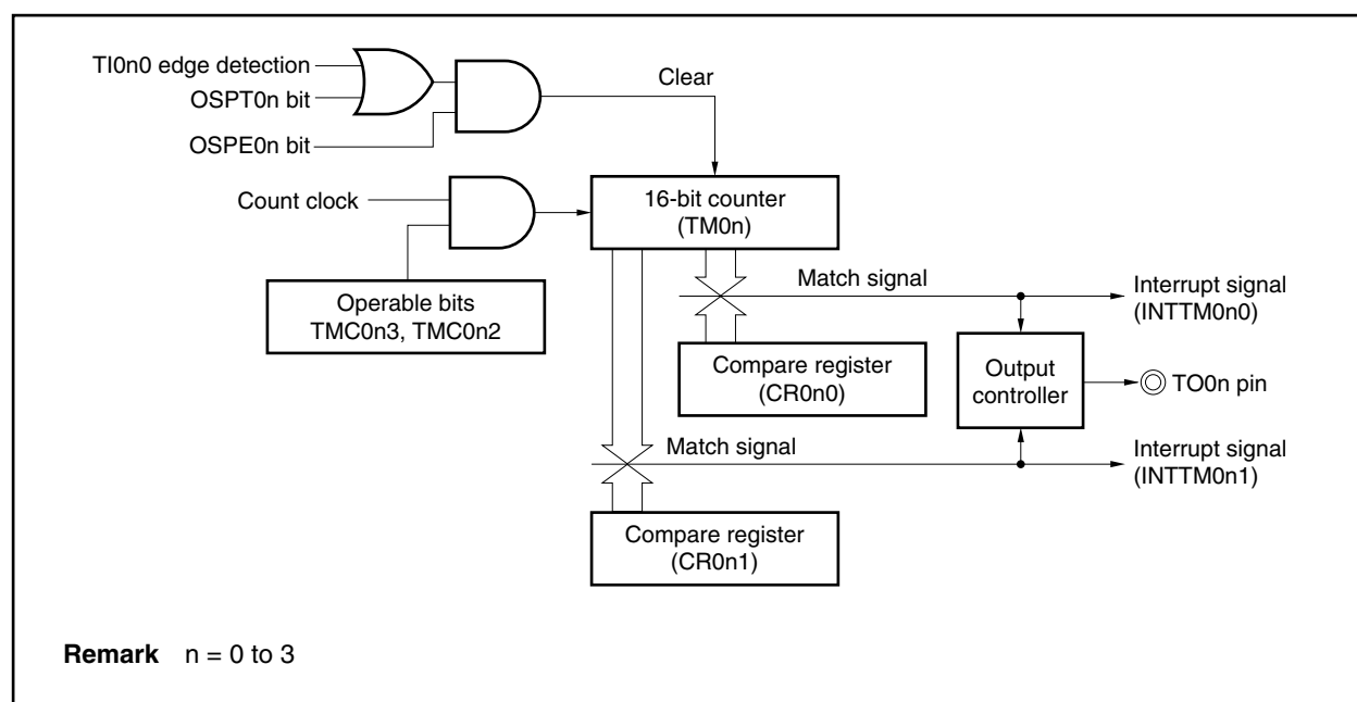
Figure 8-34. Block Diagram of One-Shot Pulse Output Operation
