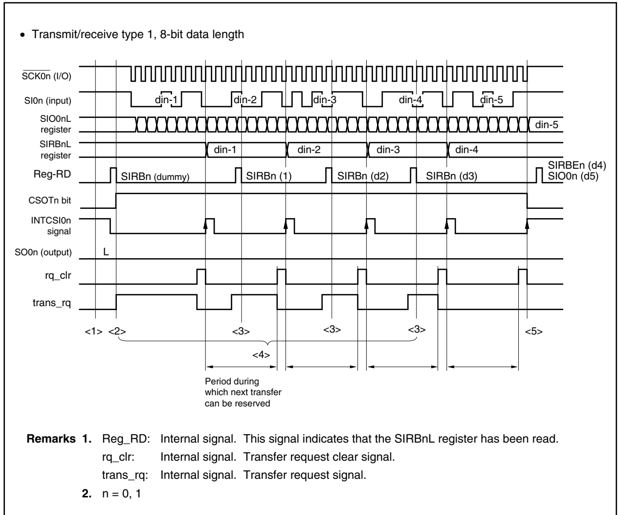
Figure 17-4. Continuous Transfer (Receive-Only) Timing Chart
