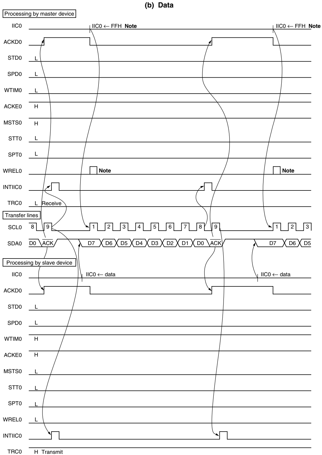
Figure 19-21. Example of Slave to Master Communication (When 8-Clock Wait for Master and 9-Clock Wait for Slave Are Selected) (2/3)
