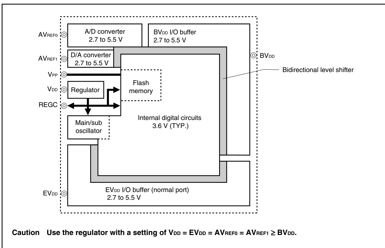
Figure 25-1. Regulator
