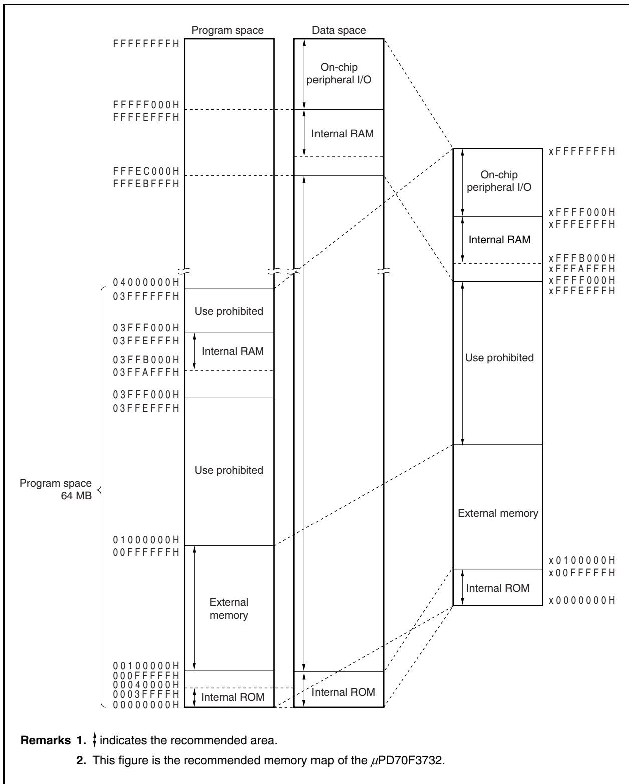
Figure 3-9. Recommended Memory Map
