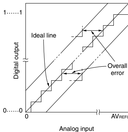
Figure 14-12. Overall Error
