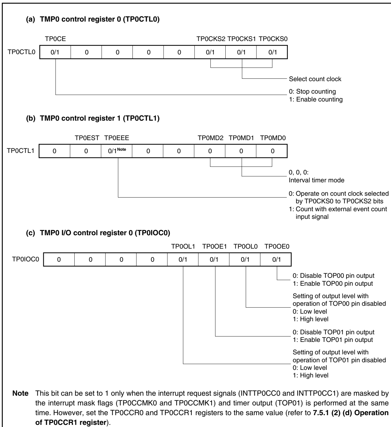
Figure 7-4. Register Setting for Interval Timer Mode Operation (1/2)
