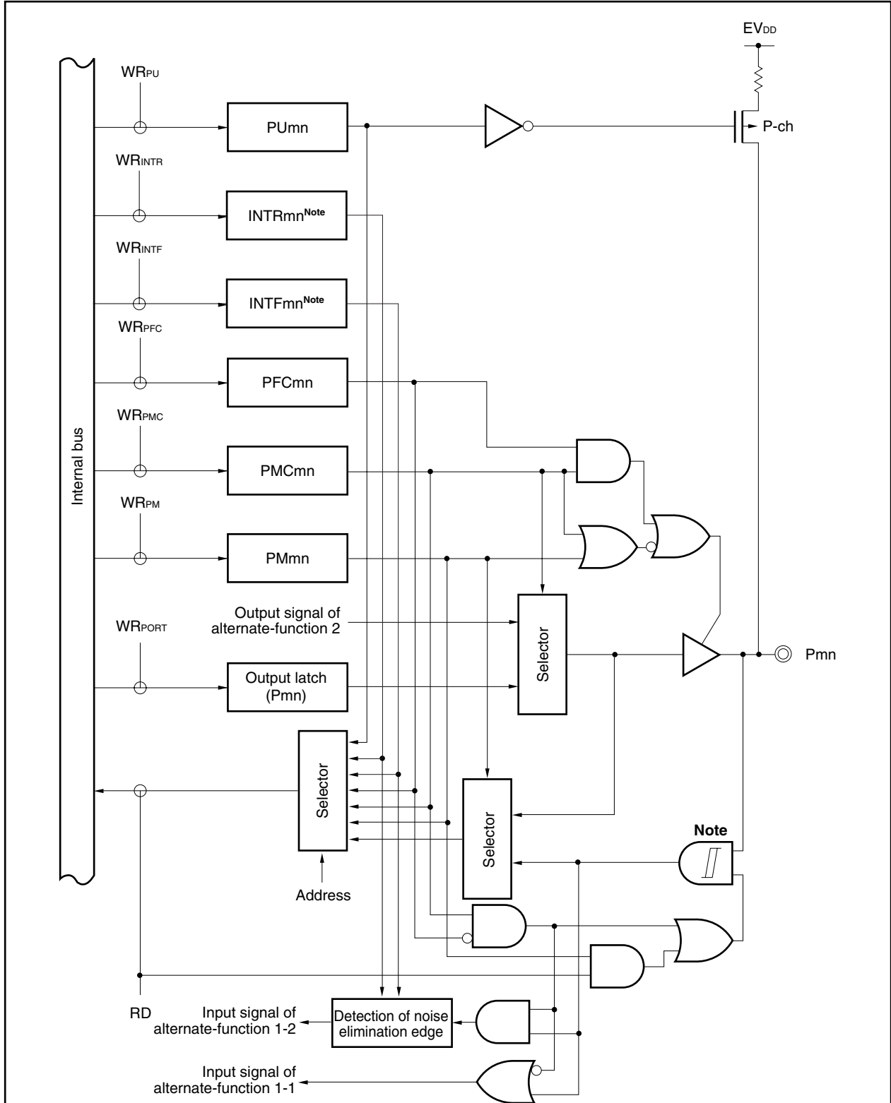
Figure 4-22. Block Diagram of Type E10-SUIHL
