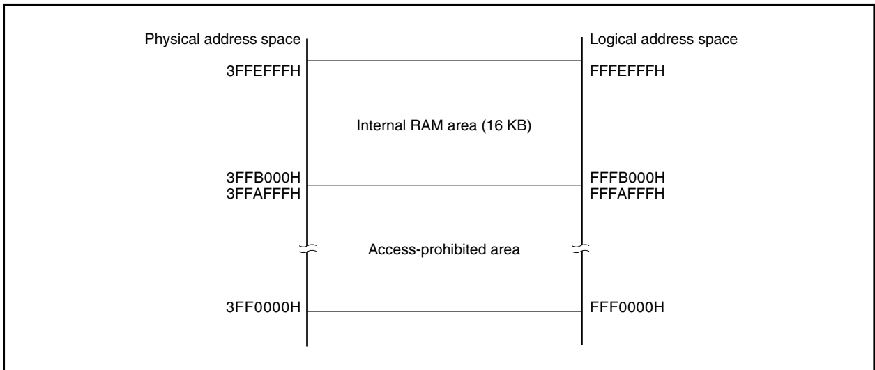
Figure 3-6. Internal RAM Area (16 KB)
