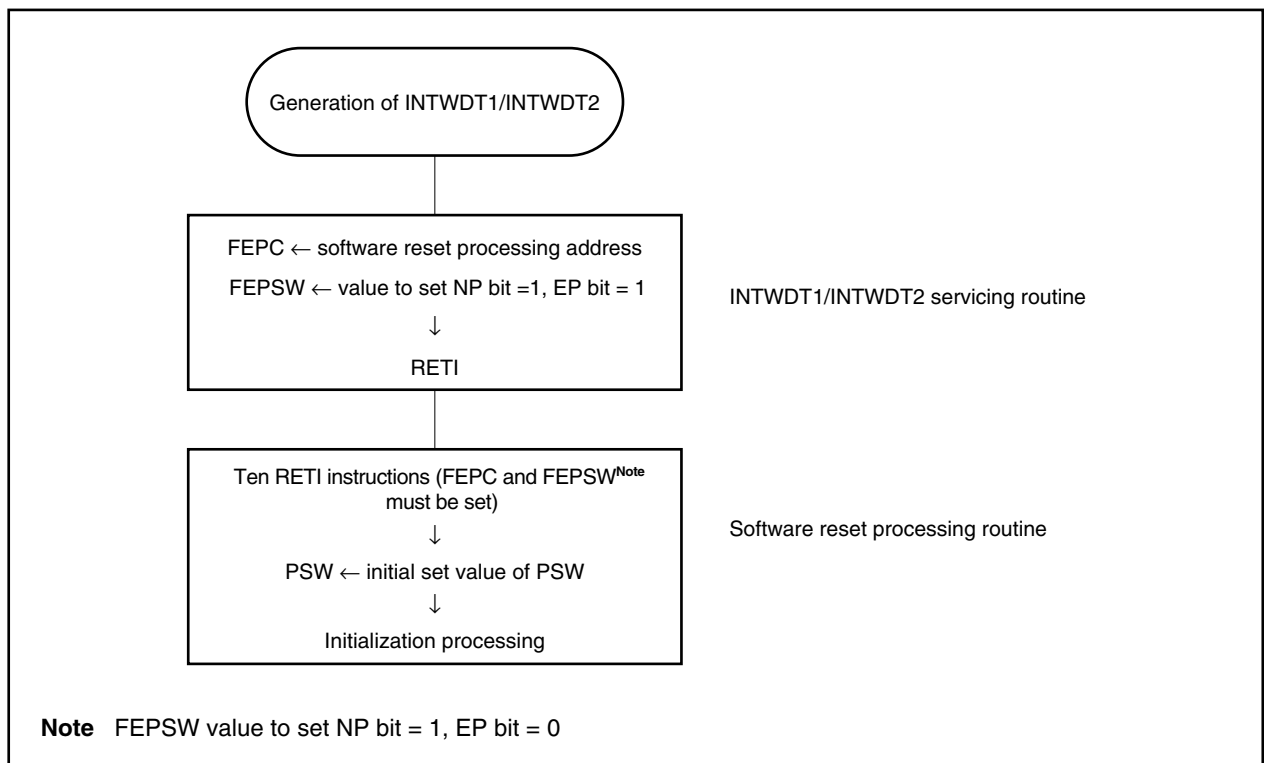
Figure 21-15. Restoring by RETI Instruction
