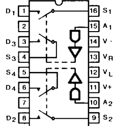
HI1-50XX/883 (CERAMIC DIP)
