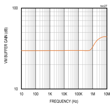
VM BUFFER GAIN vs. FREQUENCY (ABS)
