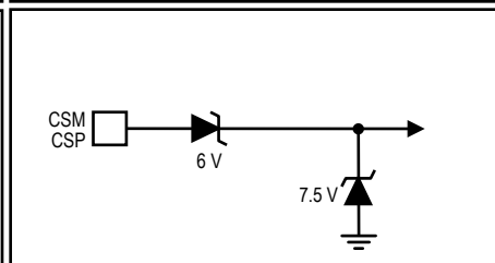
Figure 27h: Current Sense Amp Inputs
