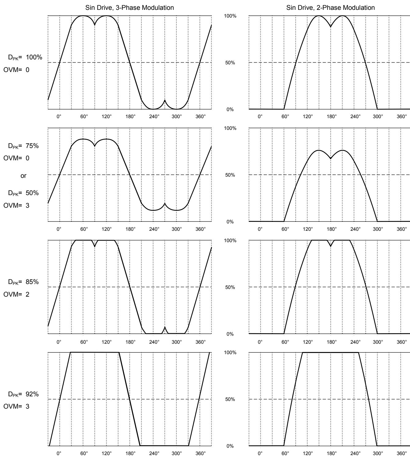
Figure 9: Modulation and Overmodulation Examples
