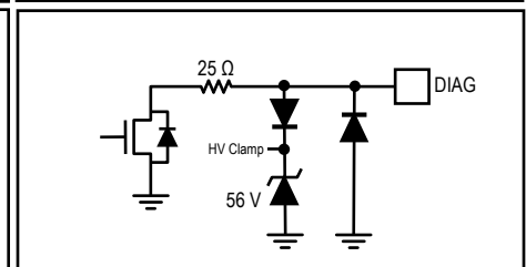
Figure 27i: HV Compliant Output
