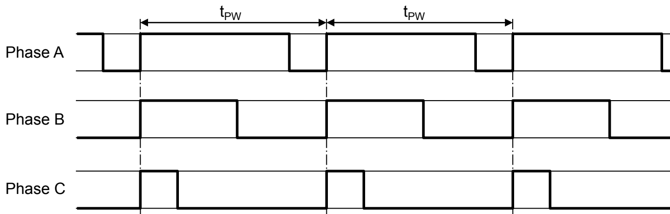
Figure 10b: Edge Aligned Bridge PWM Mode PMD = 1
