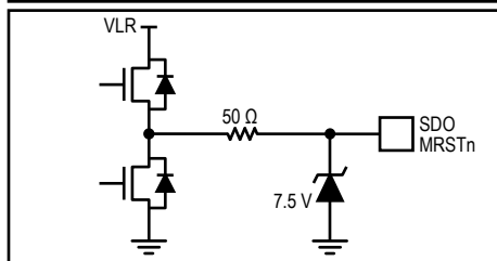
Figure 27g: Logic Output
