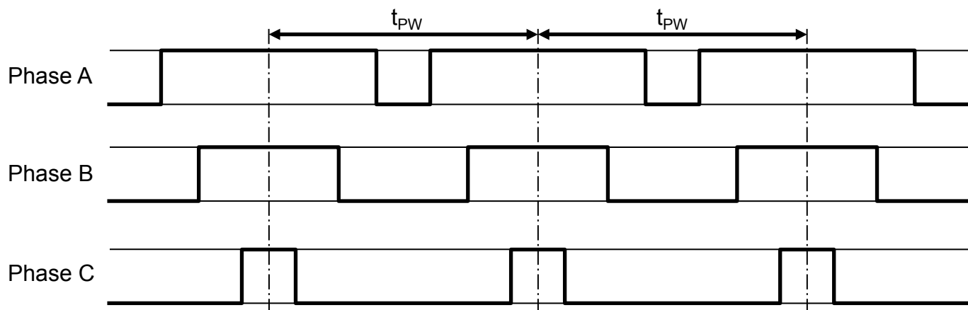
Figure 10a: Center-Aligned Bridge PWM Mode PMD = 0
