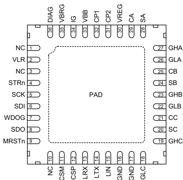
36-terminal eQFN (suffix EV)
