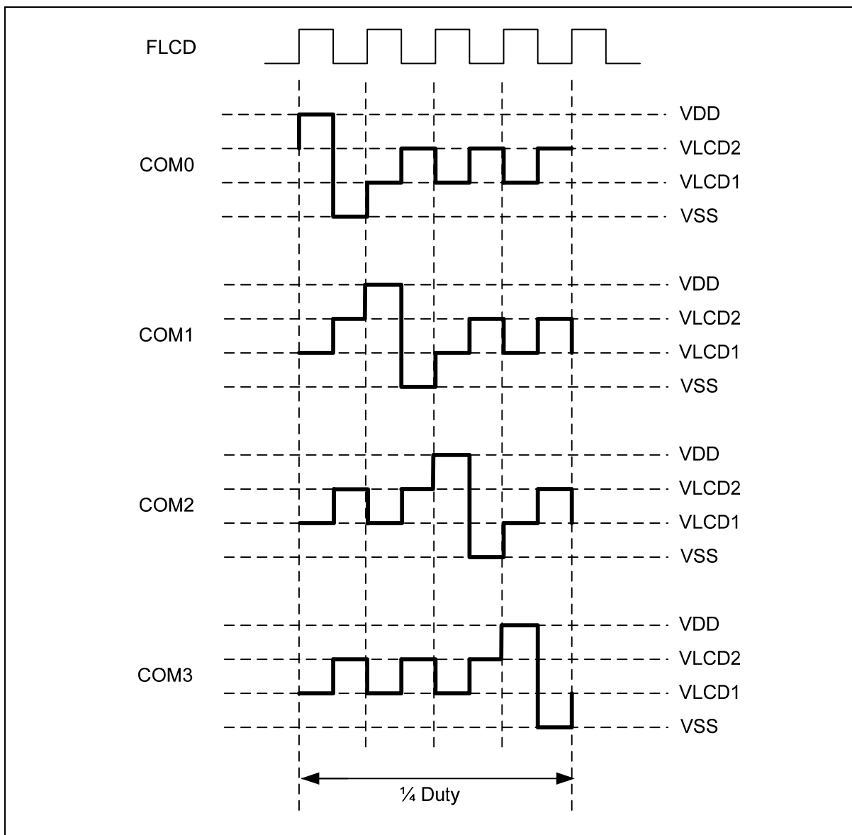
Figure 20-5: LCD com output pins configured using Voltage Pump A type with 1/4 duty.
