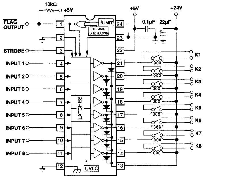
MIC59P50 Protected Relay Driver
