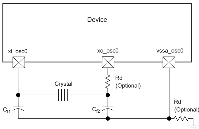
Figure 5-9. Crystal Implementation
