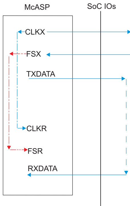
Figure 5-67. McASP1-8 CO-FI- – SYNC Mode
