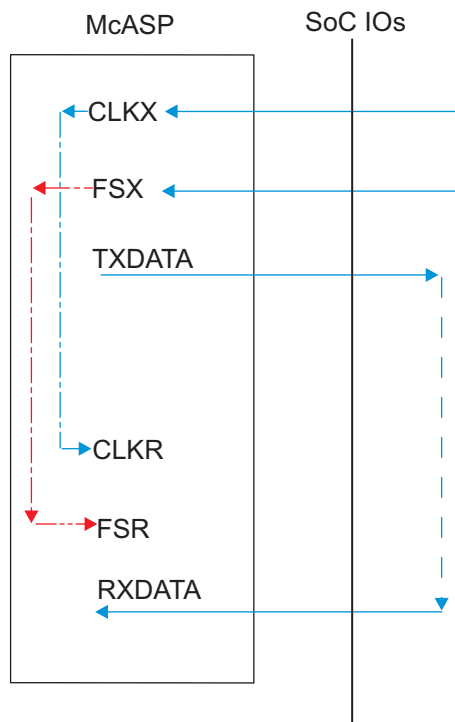
Figure 5-66. McASP1-8 CI-FI- – SYNC Mode
