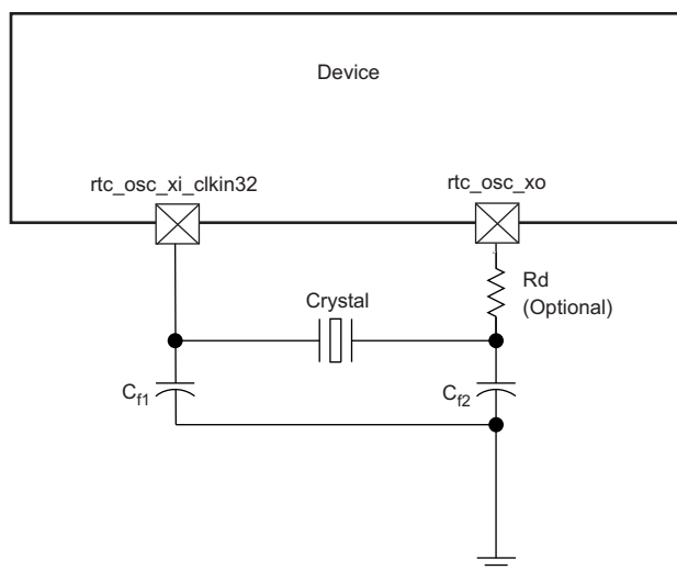
Figure 5-17. Crystal Implementation
