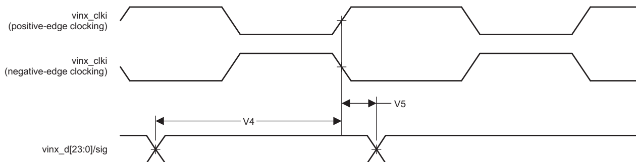
Figure 5-22. Video Input Ports Timings
