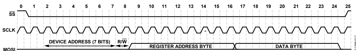
Figure 17. SPI Write to ADAU1966A Clcking
