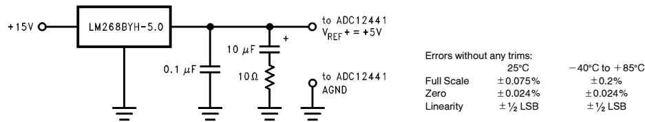
FIGURE 2b. Simple Reference Circuit
