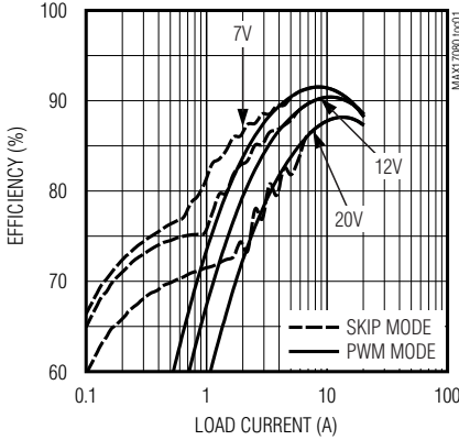
CORE SMPS 1-PHASE EFFICIENCY vs. LOAD CURRENT ( V_{OUT} = 0.8V )
