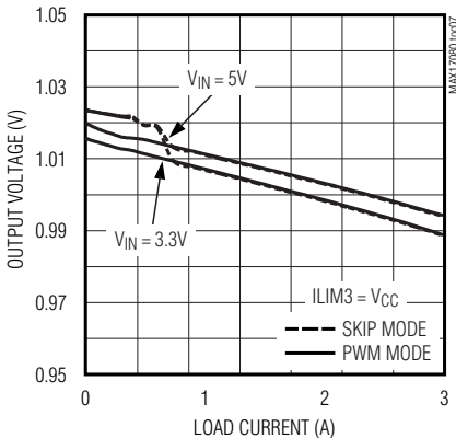
NB SMPS OUTPUT VOLTAGE vs. LOAD CURRENT ( V_{OUT} = 1.0V )
