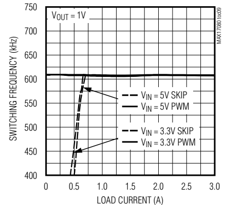
NB SMPS SWITCHING FREQUENCY vs. LOAD CURRENT
