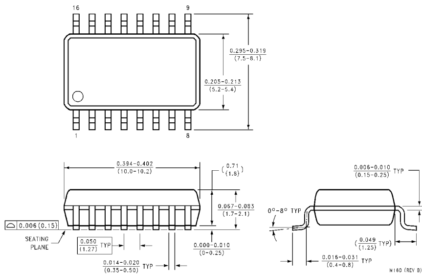
Small Outline Package (SJ) Order Number DM74ALS174SJ or DM74ALS175SJ Package Number M16D
