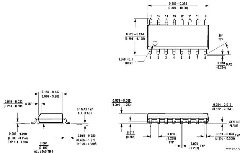
S.O. Package (M) Order Number DM74ALS174M or DM74ALS175M Package Number M16A
