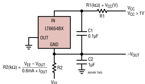
Negative Voltage Reference
