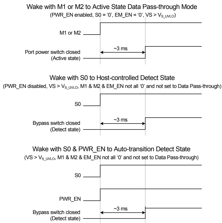
Figure 4.5 Wake Timing
