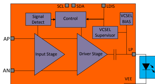
Figure 1: Device diagram
