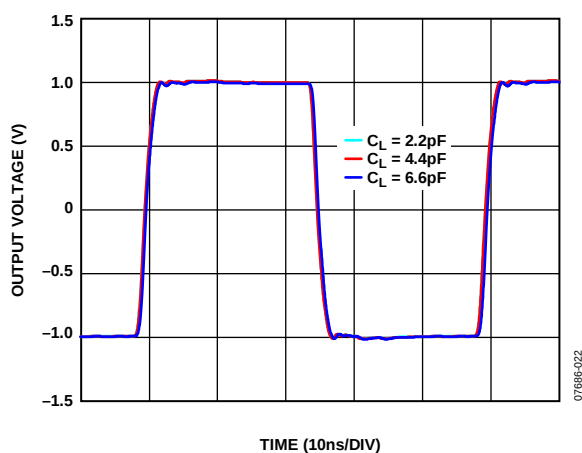
Figure 22. Large Signal Transient Response vs. Capacitive Load
