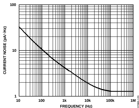
Figure 20. Output Current Noise vs. Frequency
