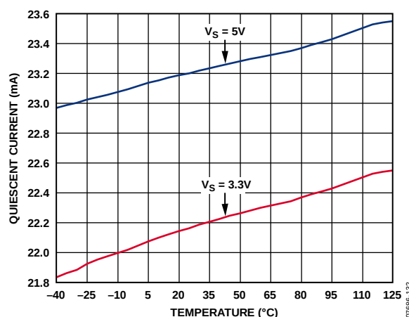
Figure 28. Quiescent Current vs. Temperature
