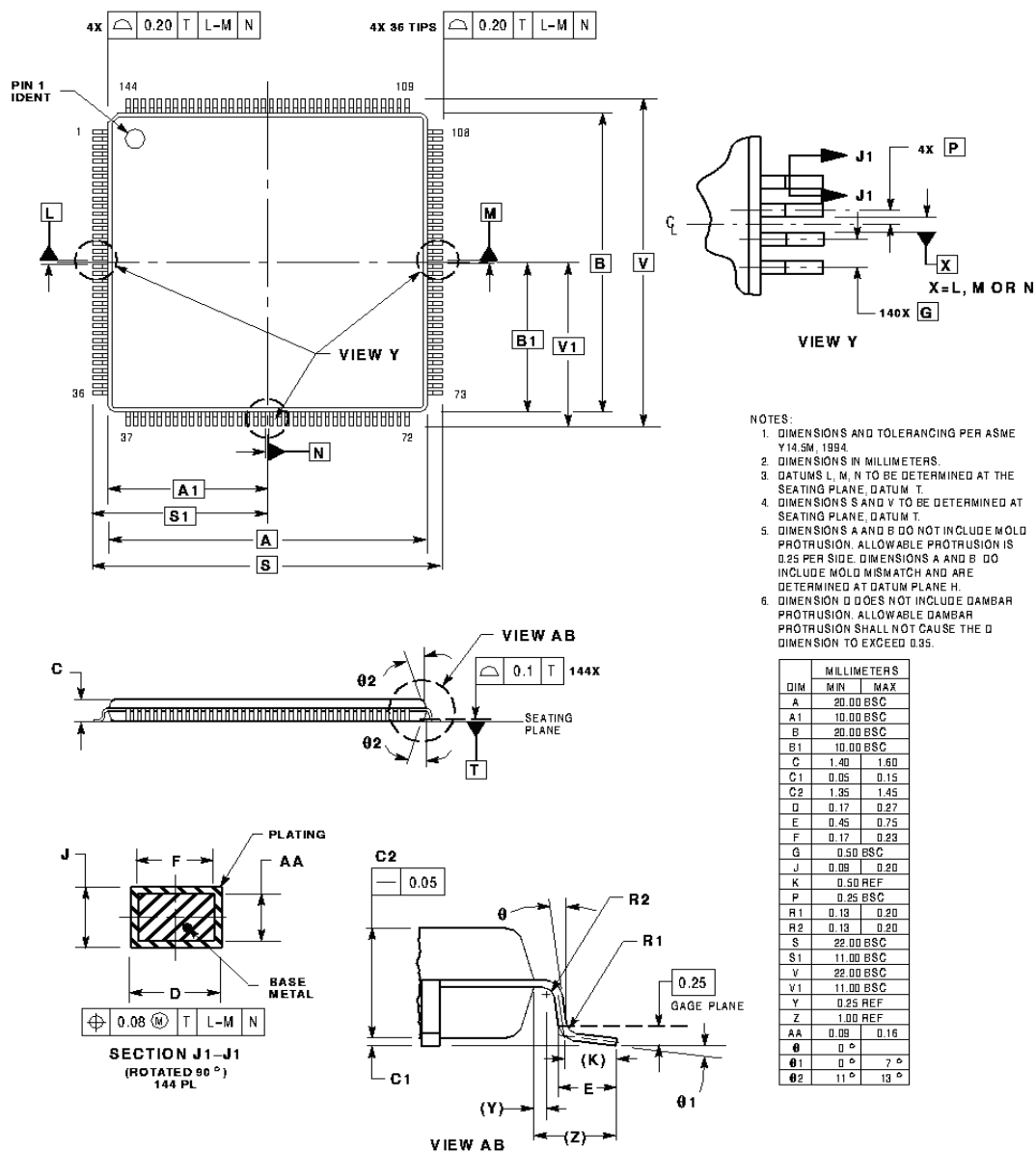
Figure 5-2 144-pin LQFP Mechanical Information
