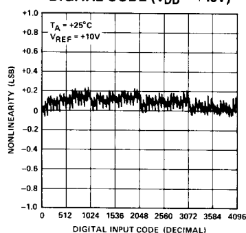
NONLINEARITY vs DIGITAL CODE ( V_{DD} = +15V )
