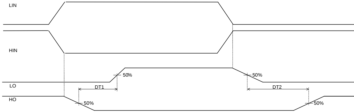
Figure 5: Deadtime definition
