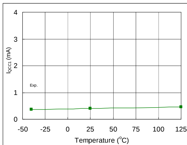
Fig. 34. Quiescent VCC Supply Current vs. Temperature
