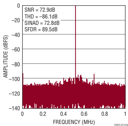
Figure 16. 32k Point FFT of the LTC2321-12
