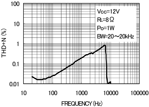
Fig. 2 THD+N — Frequency
