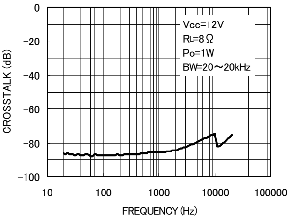
Fig. 4 Crosstalk - Frequency
