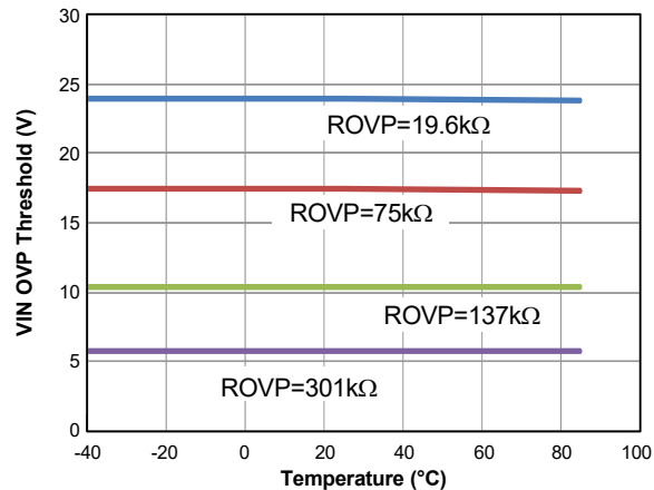
Figure 18. VIN OVP vs. Temperature ( I_{VOUT}=1\text{A} )
