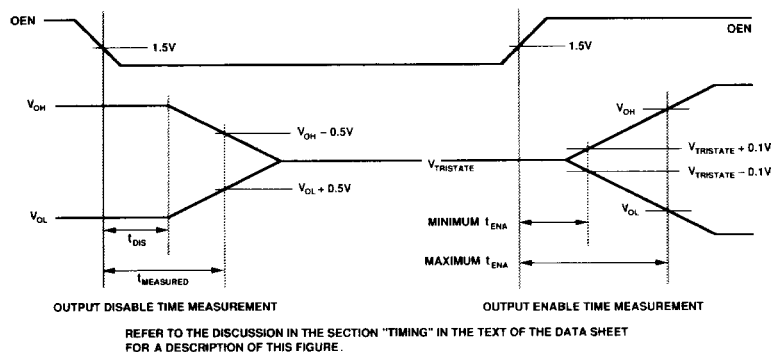
Figure 1. Three-State Disable and Enable Timing
