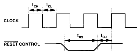
Figure 2. Reset Timing
