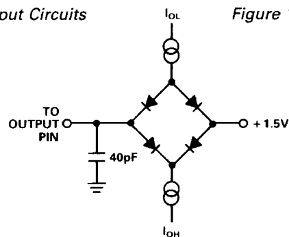
Figure 12. Normal Load for AC Measurements
