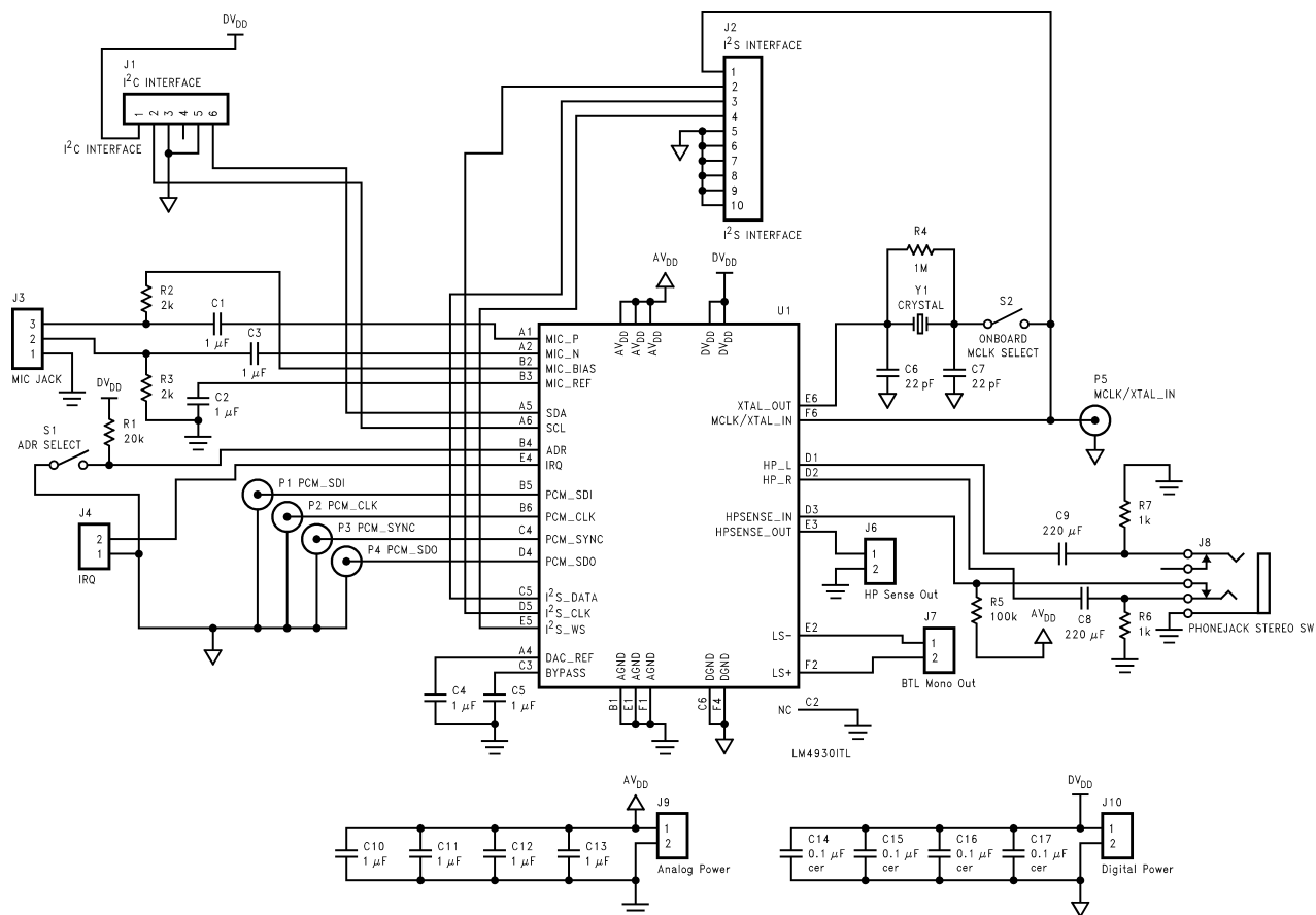
FIGURE 5. LM4930ITL Demo Board Schematic
