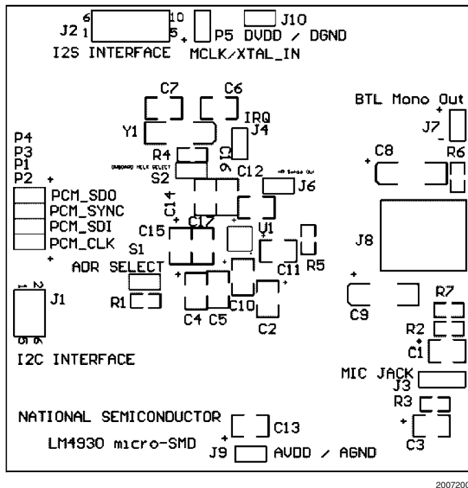
FIGURE 7. LM4930ITL Demo Board Silkscreen
