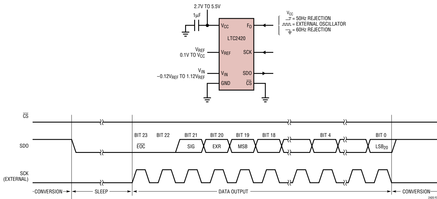
Figure 8. External Serial Clock, \overline{\text{CS}} = 0 Operation
