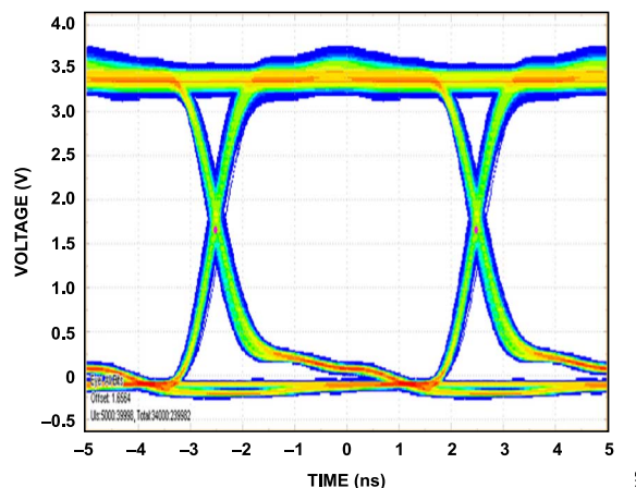
Figure 18. ADN4693E-1 Driver Output Eye Pattern ( V_{CC} = 3.3 V, T_A = 25^\circ\text{C} , Data Rate = 200 Mbps, PRBS 2^{15} - 1 Input, R_L = 50 \Omega )
