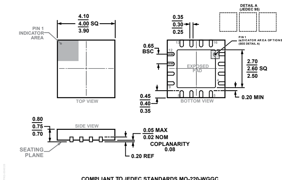
Figure 39. 16-Lead Lead Frame Chip Scale Package [LFCSP] 4 mm × 4 mm Body and 0.75 mm Package Height (CP-16-17) Dimensions shown in millimeters
