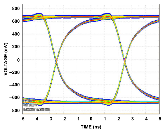
Figure 19. ADN4693E-1 Receiver Output Eye Pattern ( V_{CC} = 3.3 V, T_A = 25^\circ\text{C} , Data Rate = 200 Mbps, PRBS 2^{15} - 1 Input, C_L = 15 pF)
