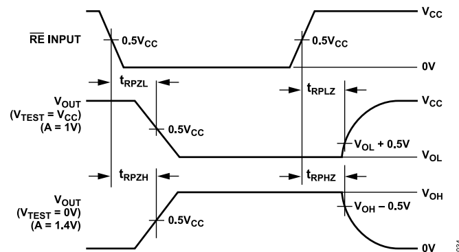
Figure 35. Receiver Enable and Disable Times
