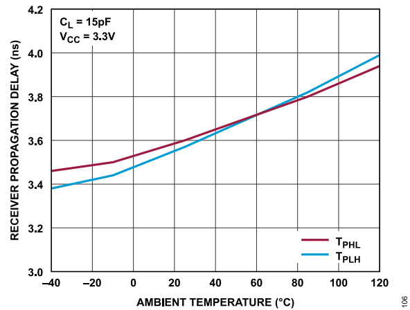
Figure 10. Receiver Propagation Delay vs. Ambient Temperature (Clock Frequency = 100 MHz, V_{ID} = 300 mV, V_{IC} = 1.1 V)
