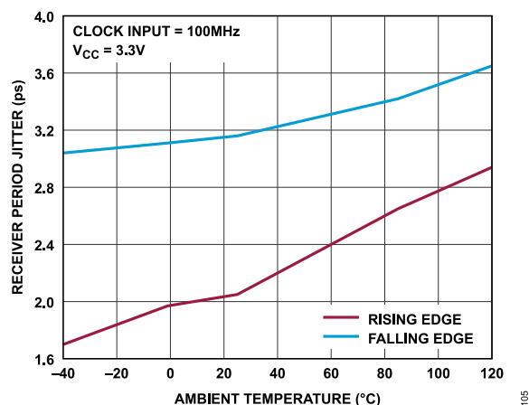
Figure 15. Receiver Period Jitter vs. Ambient Temperature ( V_{ID} = 400 mV, V_{IC} = 1.1 V)
