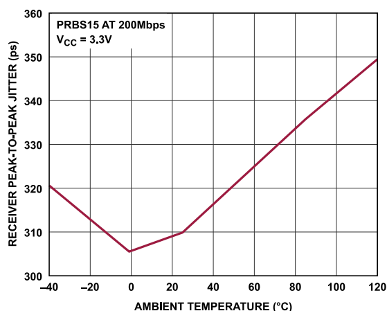
Figure 17. Receiver Peak-to-Peak Jitter vs. Ambient Temperature ( V_{ID} = 400 mV, V_{IC} = 1.1 V)
