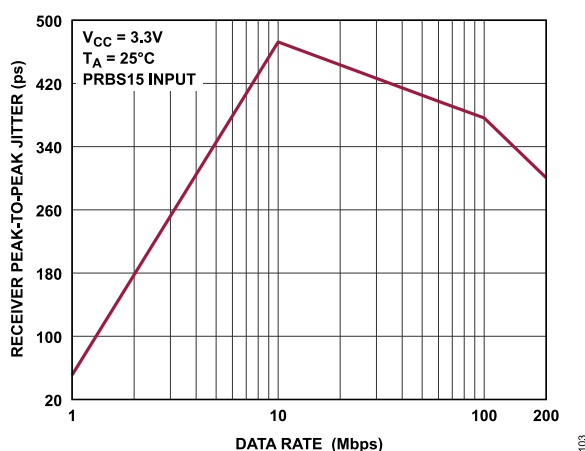
Figure 16. Receiver Peak-to-Peak Jitter vs. Data Rate ( V_{ID} = 400 mV, V_{IC} = 1.1 V)
