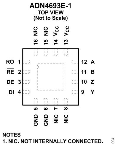
Figure 2. Pin Configuration
