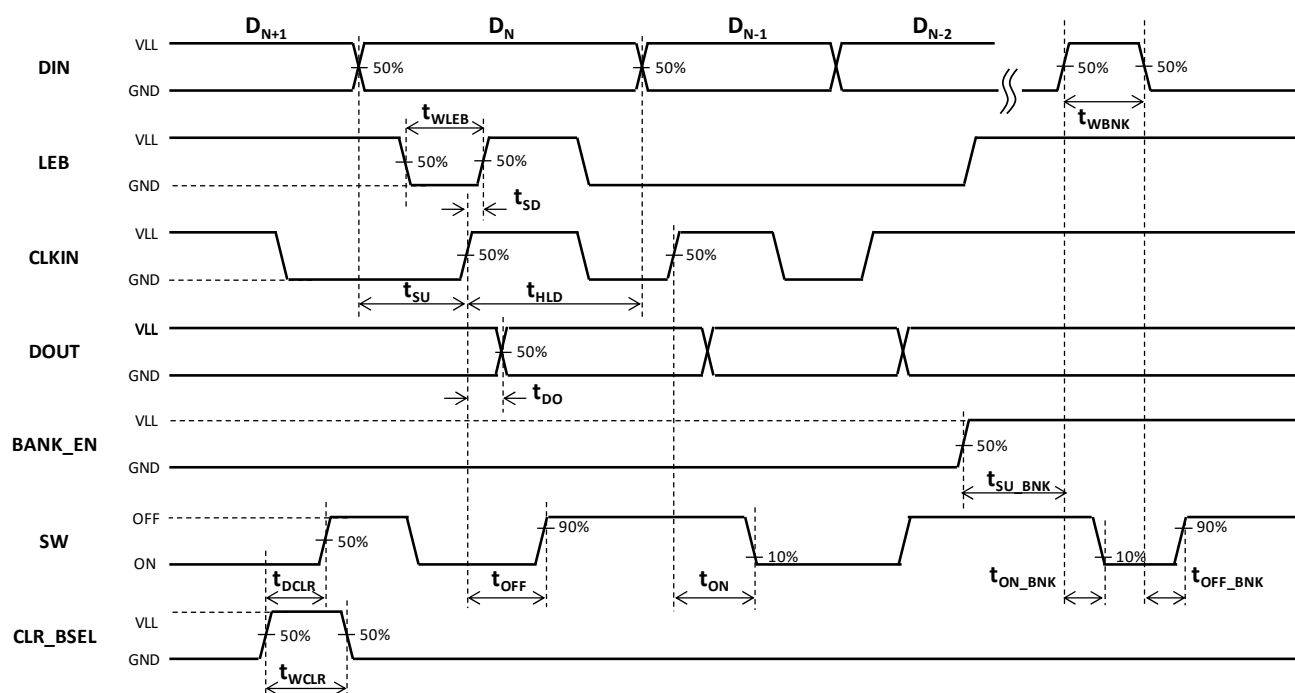
Figure 3 Logic Timing
