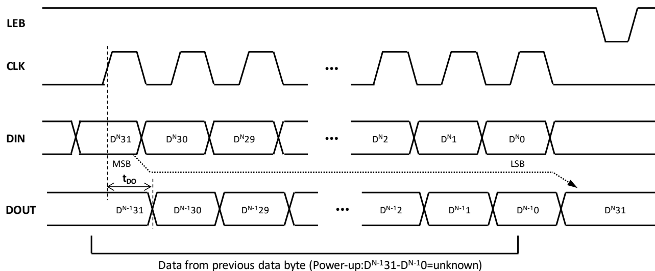
Figure 4 Latch Enable Interface Timing
