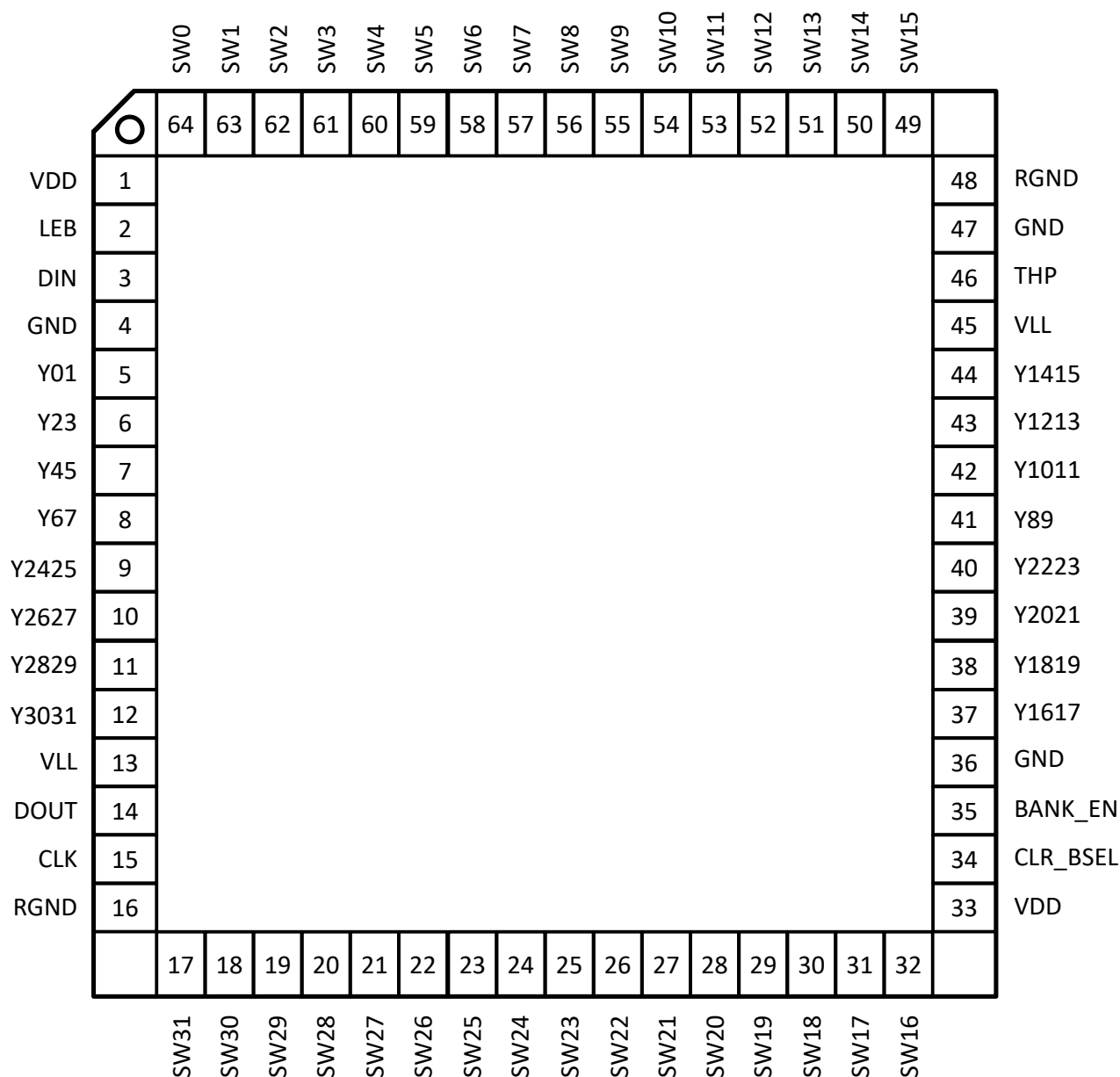
Figure 5 Pin Configuration
