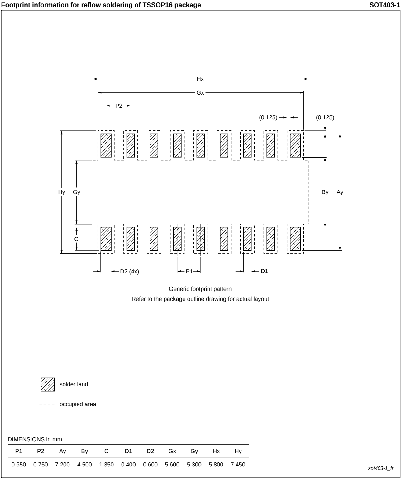
Fig 33. PCB footprint for SOT403-1 (TSSOP16)
