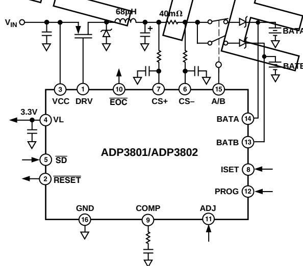
Figure 1. 4 Amp Dual Battery Charger
