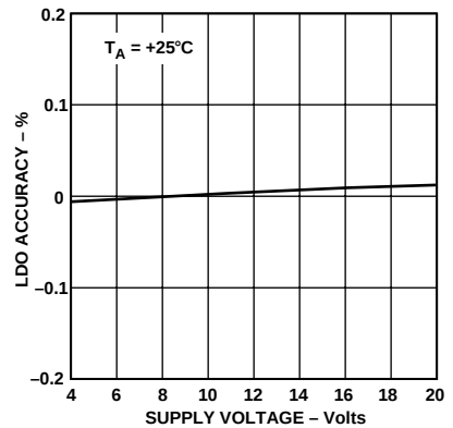
Figure 10. LDO Accuracy vs. Supply Voltage
