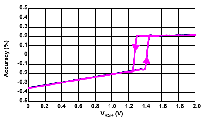
Figure 28. Gain Accuracy vs V_{RS+} = 0V to 2V
