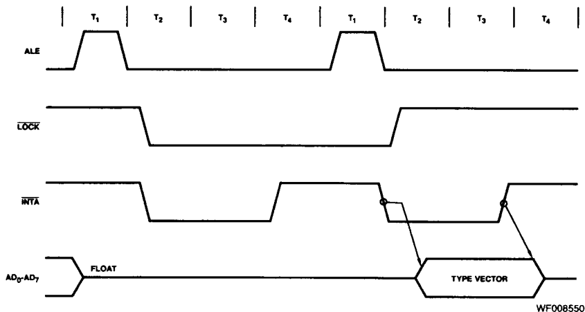
Figure 1. Interrupt Acknowledge Sequence
