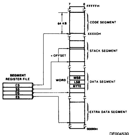
Figure 2. Memory Organization
