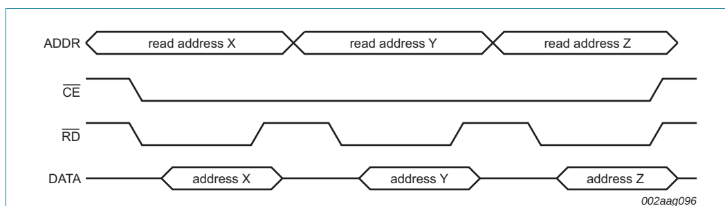
Fig 7. During normal operation, \overline{CE} may remain LOW while \overline{RD} transitions during multiple reads
