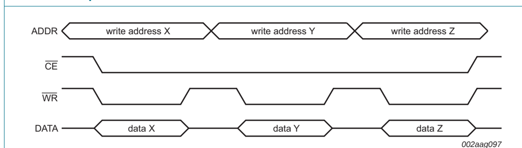
Fig 8. During normal operation, \overline{CE} may remain LOW while \overline{WR} transitions during multiple writes
