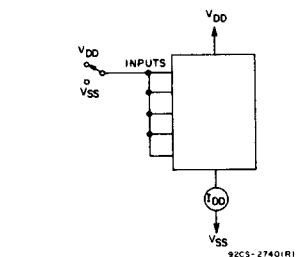
Fig. 14 - Quiescent-device-current test circuit.
