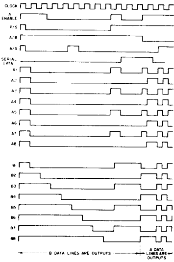
Fig. 4 — Timing diagram.
