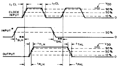
* INPUT REFERS TO ANY OF THE "A" OR "B" DATA INPUTS, "A" ENABLE, SERIAL INPUT, A/B, P/S, OR A/S INPUTS ** t_{SLH} AND t_{SHL} ARE SET-UP TIMES
