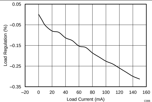
Figure 16. Load Current vs Load Regulation
