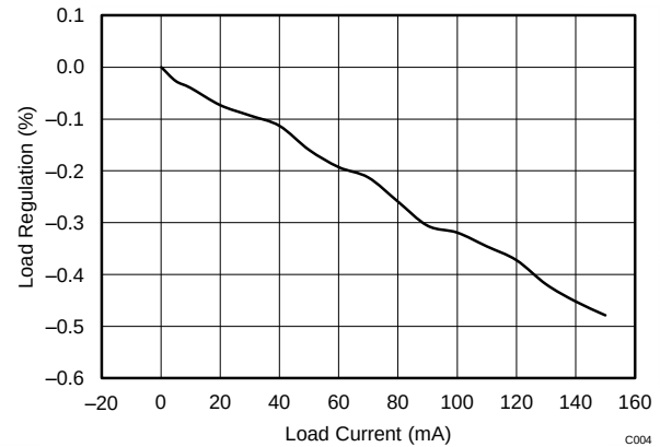
Figure 14. Load Current vs Load Regulation
