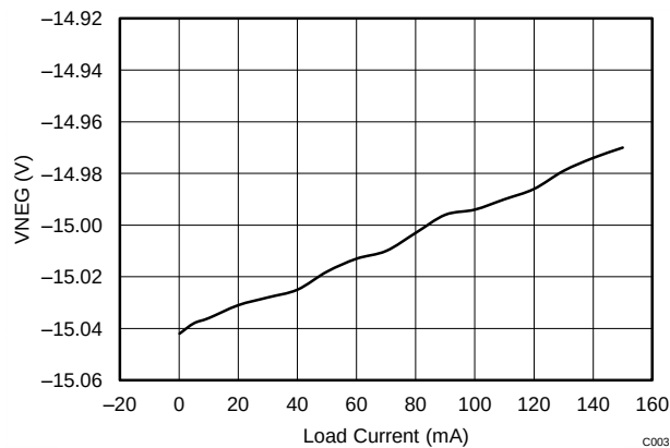
Figure 13. Load Current vs VNEG
