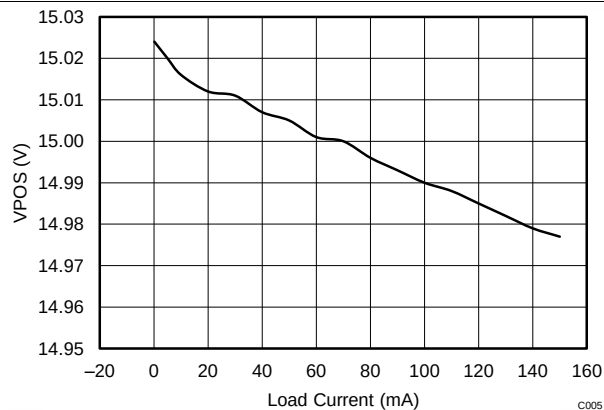
Figure 15. Load Current vs VPOS
