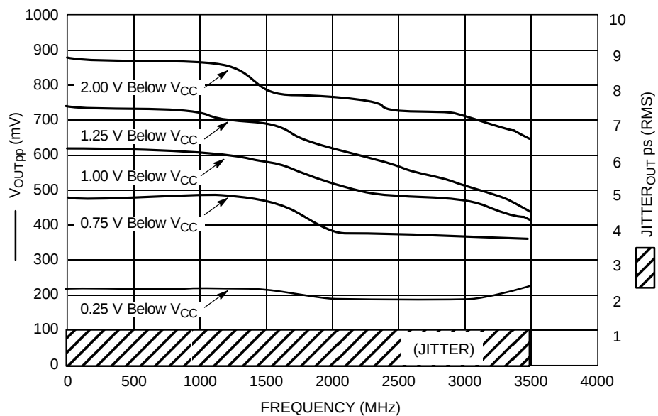
Figure 8. F_{max} /Jitter
