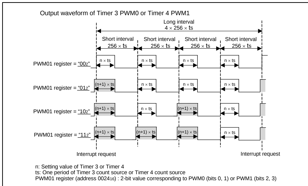
Fig. 26 Waveform of PWM0 and PWM1
