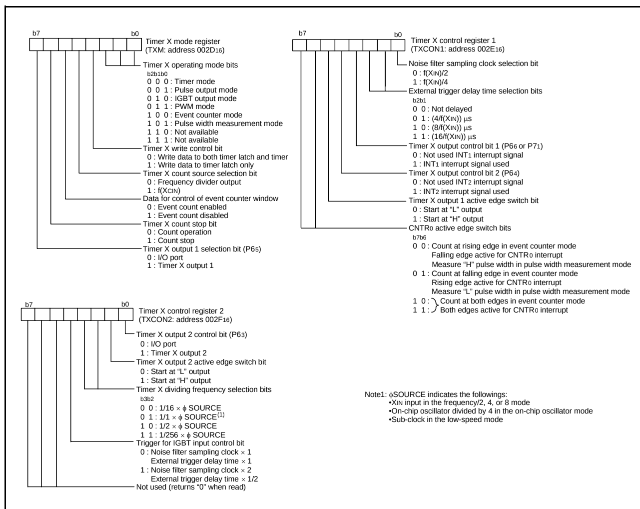
Fig. 30 Structure of Timer X related registers
