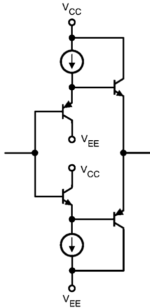
FIGURE 6. Output Stage
