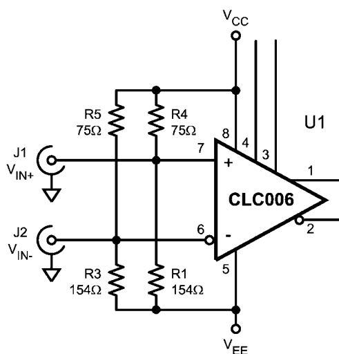
FIGURE 5. Differential 50Ω ECL Input
