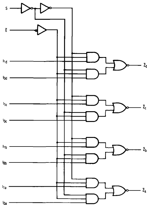
LOGIC DIAGRAM
