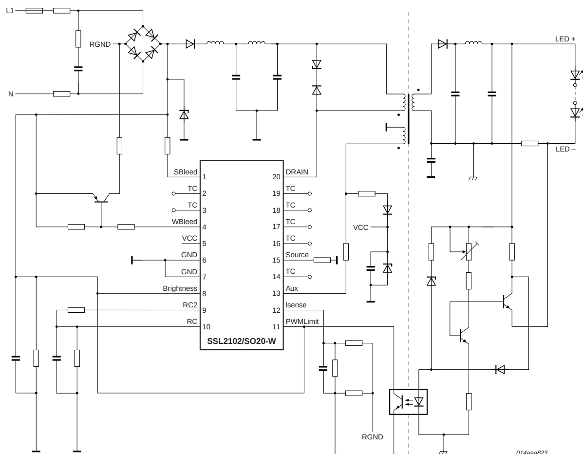
Fig 12. Application example SSL2102
