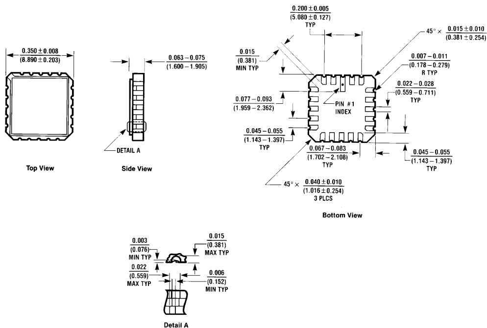
Ceramic Leadless Chip Carrier Package (E) Order Number 54LS244LMQB NS Package Number E20A
