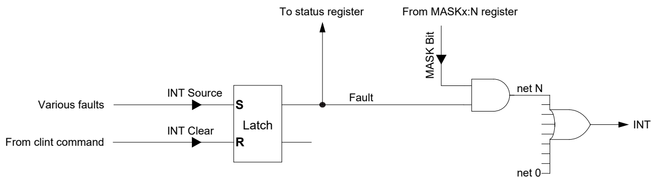
Figure 18. Interrupt handling
