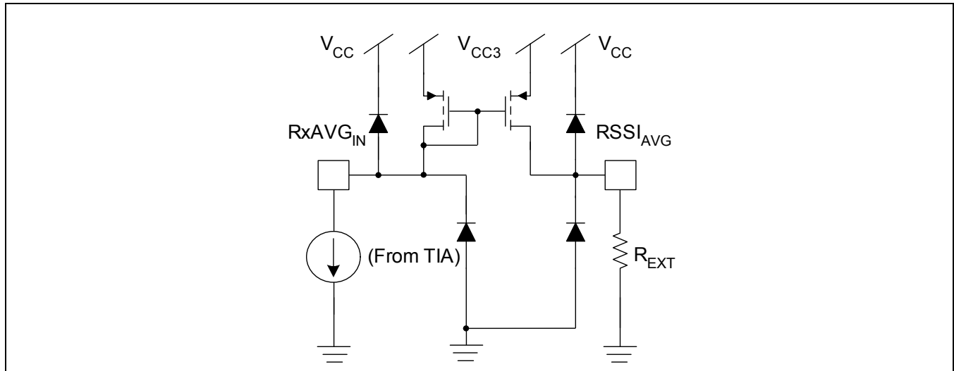
Figure 3-11. RSSI_{AVG} Output
