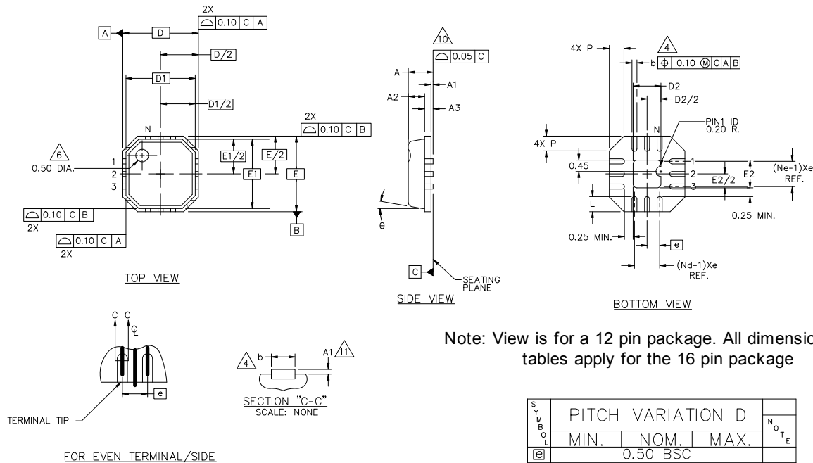
Figure 5-1. Package Information
