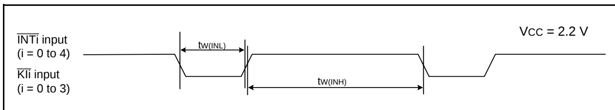
Figure 5.15 Input Timing for External Interrupt \overline{\text{INT}}_i and Key Input Interrupt \overline{\text{K}}_i when V_{cc} = 2.2 \text{ V}
