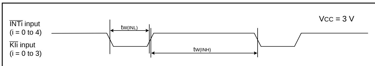
Figure 5.11 Input Timing for External Interrupt \overline{\text{INTi}} and Key Input Interrupt \overline{\text{Kli}} when Vcc = 3 V
