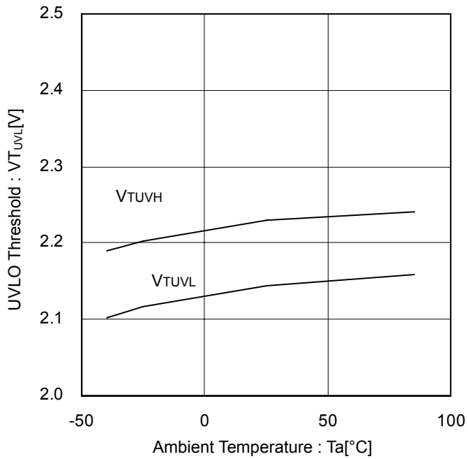
Figure 18. UVLO Threshold vs Ambient Temperature
