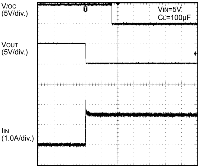
Figure 37. Over-Current Response 1ΩLoad Connected at Enable
